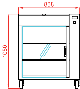
Heated Base Cabinet (1,055kW) (Optional)
